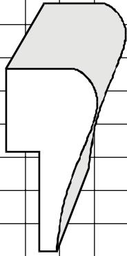
WM290 11/16" X 1-3/8"
