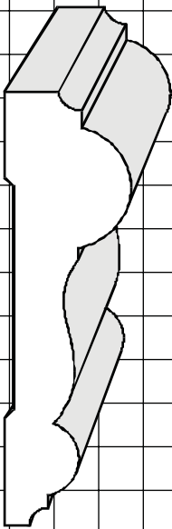
WM298 11/16" X 2-1/2"
