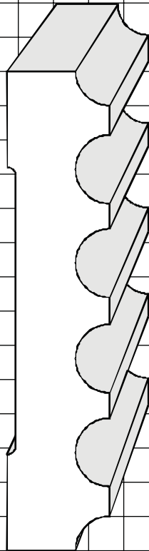
WM2004 3/4" X 3-1/2"
