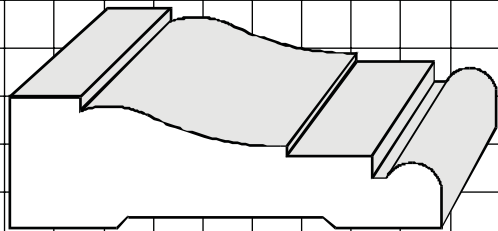
WM376 11/16" X 2-1/4"
