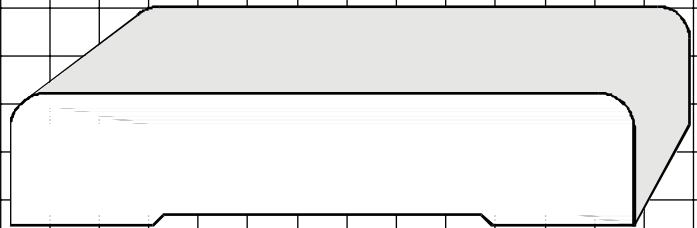
WM413 11/16" X 3-1/4"
