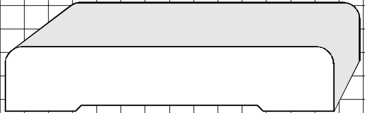
WM412 11/16" X 3-1/2"
